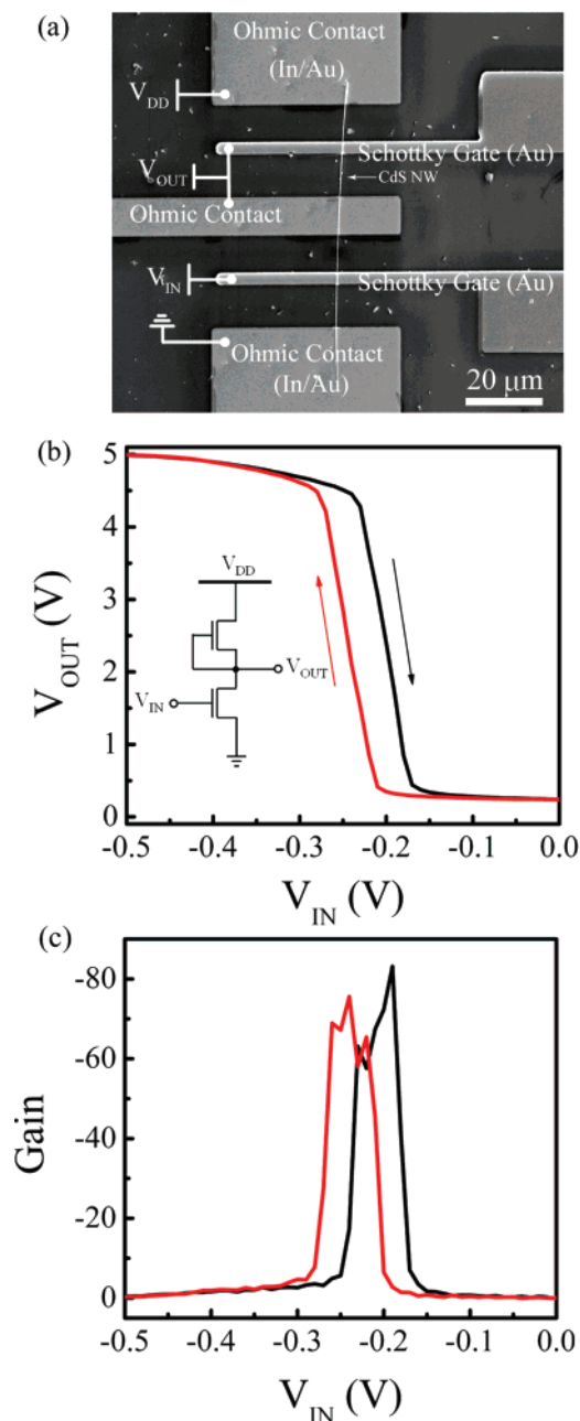
Figure 4. (a) ESEM image of an inverter made on one single CdS NW. (b) Transfer characteristic of the inverter depicted in (a). Inset: the circuit diagram of the inverter. (c) The gain of the inverter vs the input voltage. A maximum voltage gain of 83 is obtained.
