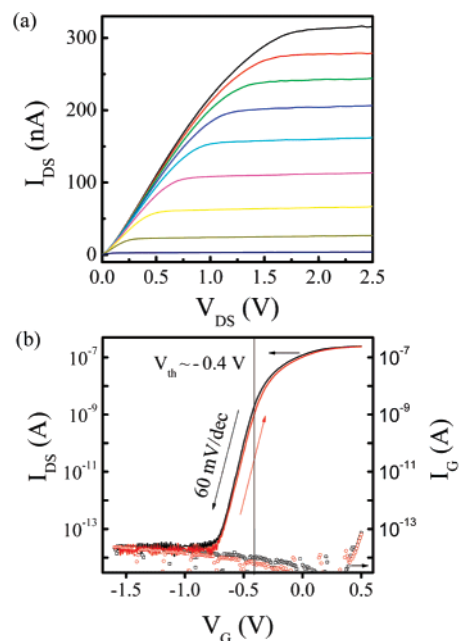
Figure 3. Performance of a single CdS NW MESFET. (a) I_{DS} – V_{DS} curves with V_G changing from 0.5 to –0.5 V, step by 0.125 V. (b) I_{DS} – V_G and I_G – V_G curves measured at V_{DS} = 1 V on an exponential scale. The arrows indicate the gate voltage sweeping direction.
